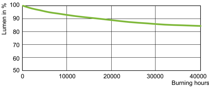
Lumen Maintenance Diagram - MST SON-T APIA Plus Xtra 100W E40 1SL/12
