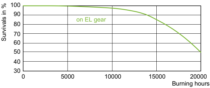
Life Expectancy Diagram - MASTERC CDM-T Elite 100W/930 G12 1CT/12
