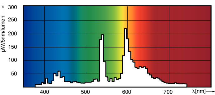
Spectral Power Distribution Colour - MC CDM-Tm Elite Mini 20W/830 GU6.5 1CT
