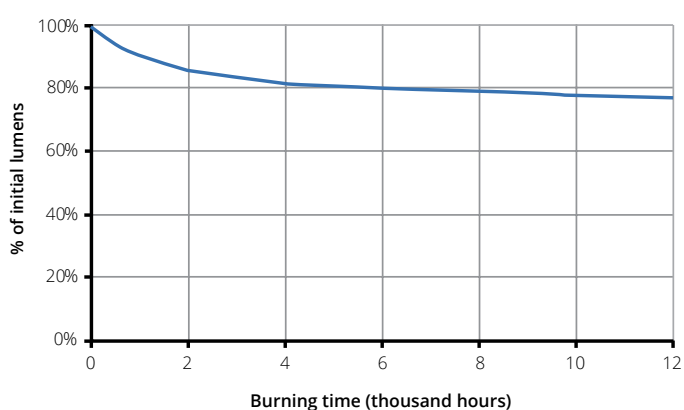
Lumen maintenance CMH G12 150W 3000K
