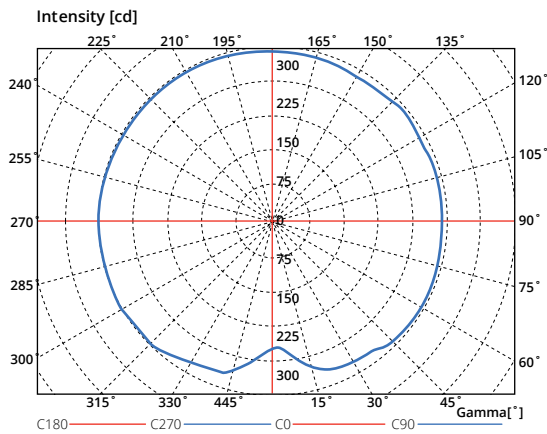
Horizontal plane polar intensity curve
