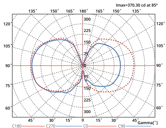
Vertical plane polar intensity curve
