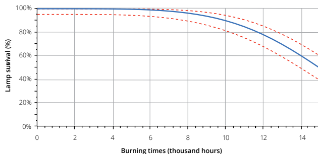
LampSurvival CMH TD 35W 3000K
