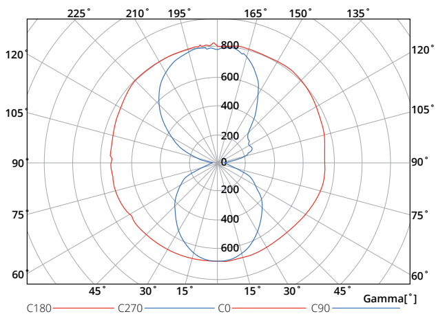
Intensity [cd]
