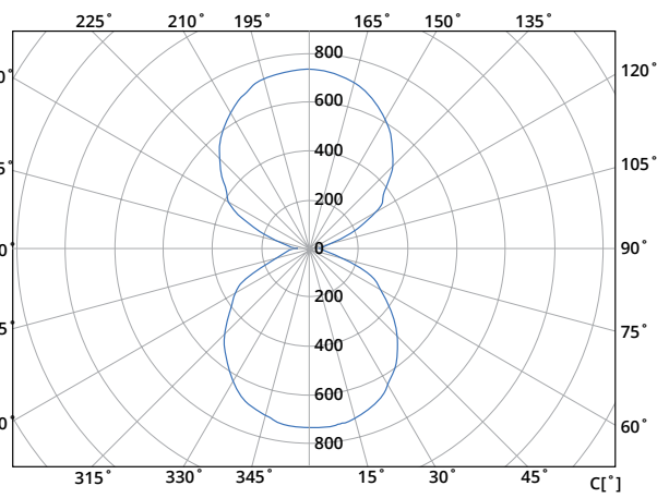
Intensity [cd]
