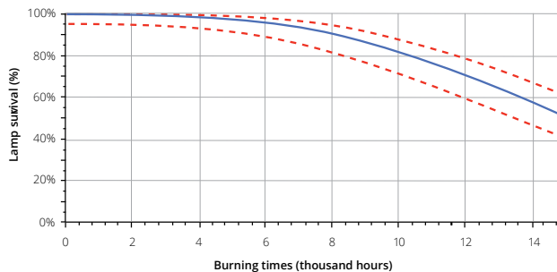
LampSurvival CMH TD 70W &amp; CMH TD 150W
