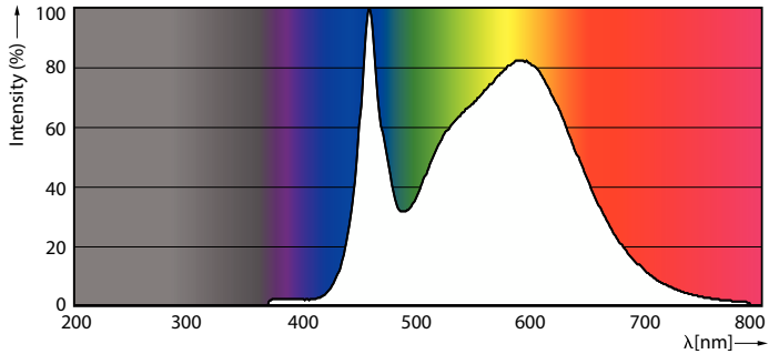
Spectral Power Distribution Colour - TForce Core LED HPL 26W E27 840 FR
