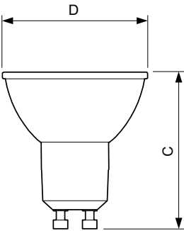
CoreProLEDspot 4-50W GU10 830 36D DIM UK
