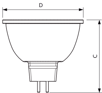
MASTER LED ExpertColor 6.7-35W MR16 940 60D
