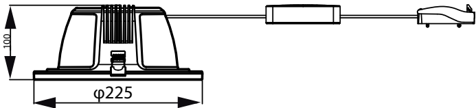
Dimensional drawing
