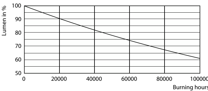
Lumen Maintenance Diagram - MAS LED SON-T IF 6Klm 34W 740 E27
