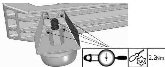
EXTERNAL SRB
