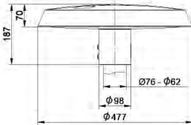
TOWNTUNE CENTRAL POST-TOP (Wind surface 0,042m 2 / SCx 0,033m 2 )
