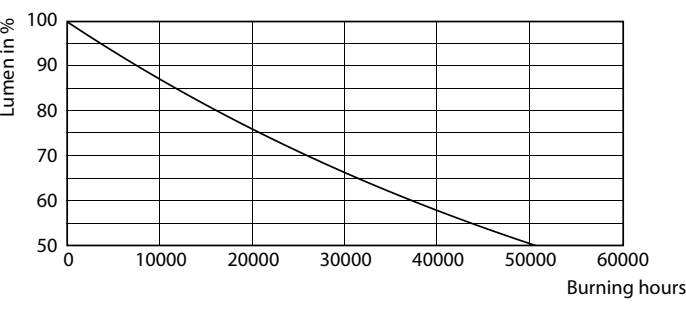
Lumen Maintenance Diagram - TForce Core LED HPL 24.5W E27 840 FR
