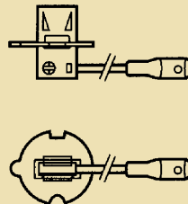
PKY 22s CH3
