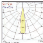
21° engstrahlend
