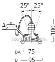
75 Swing IP44 indoor/outdoor Mindesteinbaumaße: 200x200x100mm
