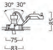
Inset Trend Swing
