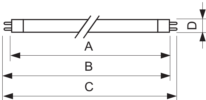
MASTER TL5 HE 14W/830 1SL
