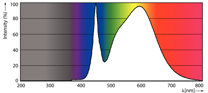
LEDtube CorePro PLL HF 24W 2G11 840 24D ND
