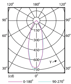
CorePro LEDspotMV 50W GU10 830 36D CLA
