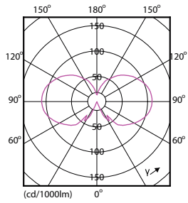
LEDbulb 100W E27 827 CL A67
