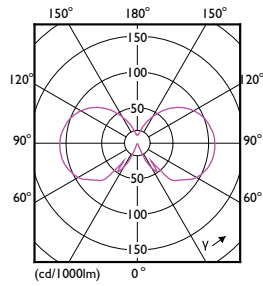
LEDbulb 60W E27 827 CL A60 ND
