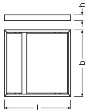
Panel Accessory 625 Surface mount kit
